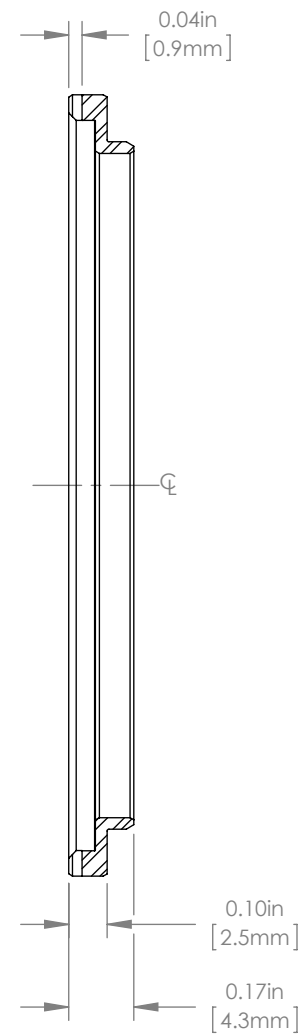
SECTION X-X
